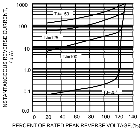
FIG.5-TYPICAL REVERSE CHARACTERISTICS
