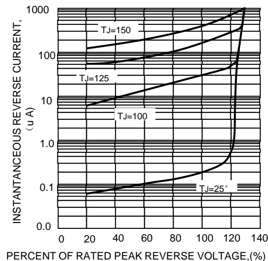
FIG.5-TYPICAL REVERSE CHARACTERISTICS
