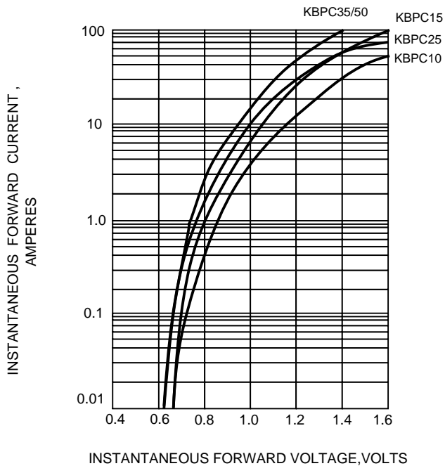
FIG.3-TYPICAL FORWARD CHARACTERISTICS
