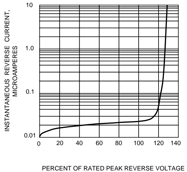
FIG.4-TYPICAL REVERSE CHARACTERISTICS
