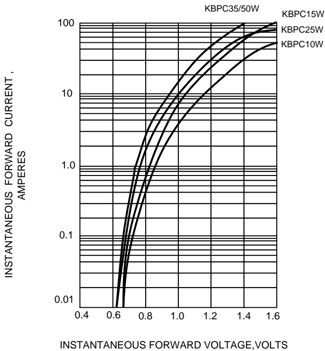
FIG.3-TYPICAL FORWARD CHARACTERISTICS
