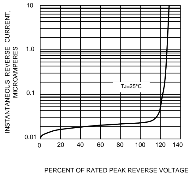
FIG.4-TYPICAL REVERSE CHARACTERISTICS
