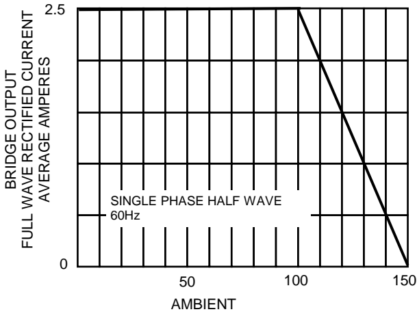
FIG.1-DERATING CURVE FOR
