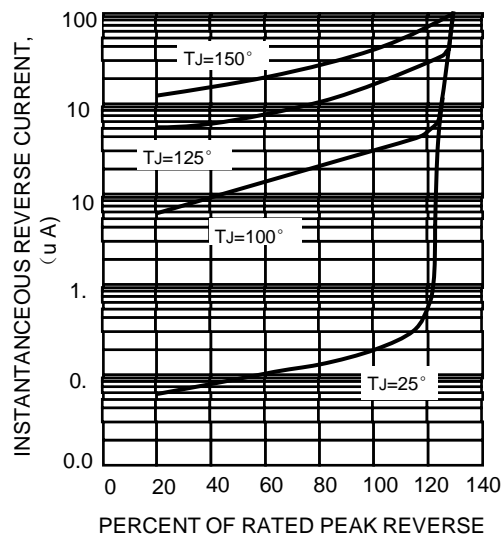
FIG.5-TYPICAL REVERSE
